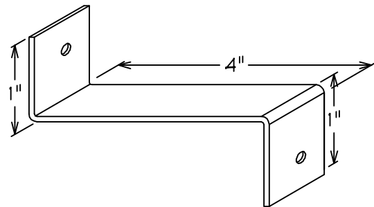
ENLARGED VIEW OF MOUNTING BRACKET
