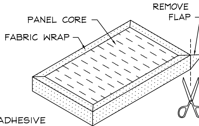
④ PANEL FACE DOWN
