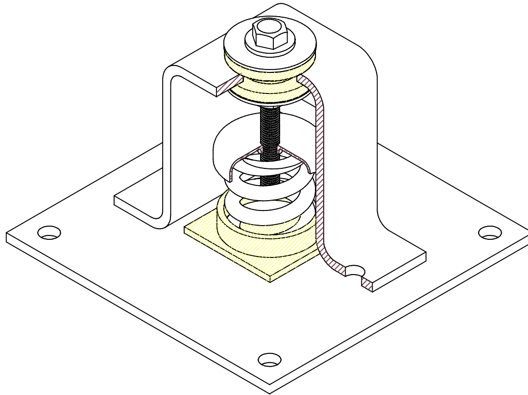
FHS ISOLATOR WITH OPTIONAL OVERSIZED BASEPLATE ASHRAE TYPE 4
