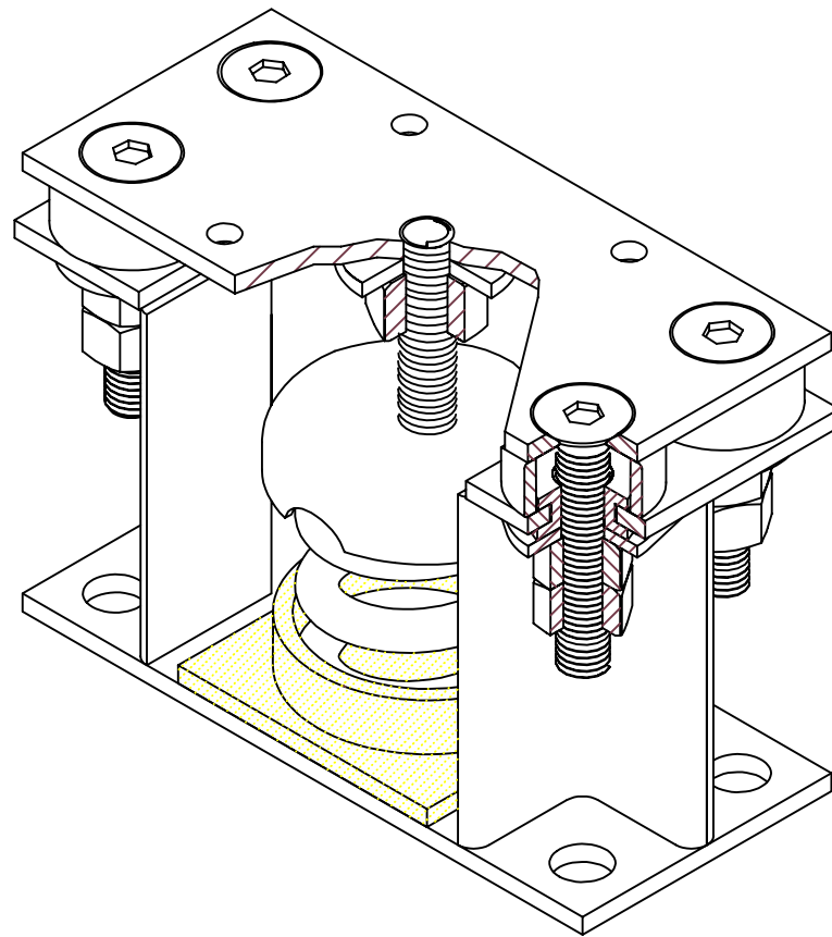
FLSS ISOLATOR ASHRAE TYPE 4
