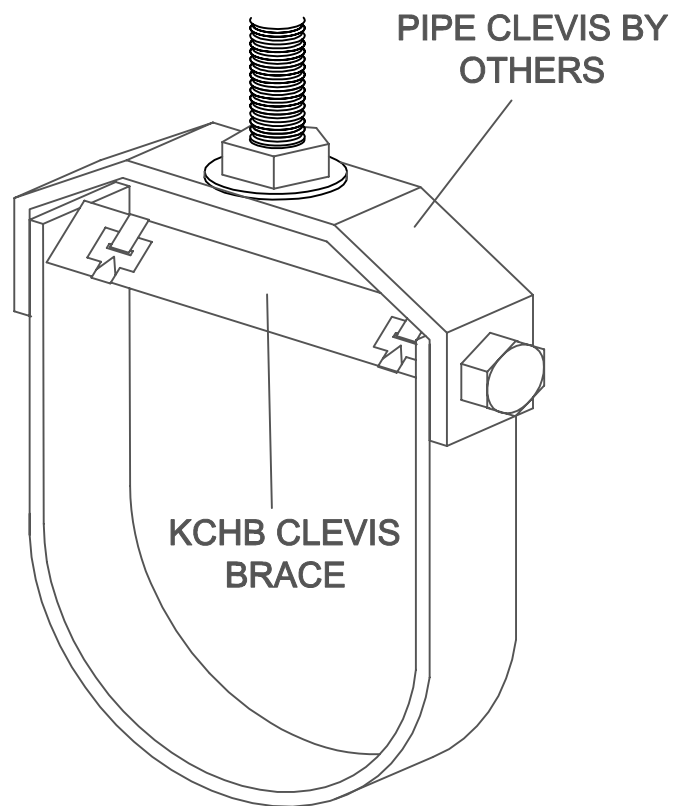
KCHB CLEVIS BRACE ASHRAE TYPE J APPLICATIONS
