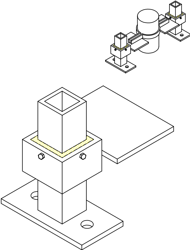
KPG RISER GUIDE ASHRAE TYPE 2
