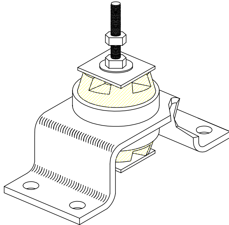
KRMS SEISMIC NEOPRENE MOUNT ASHRAE TYPE E
