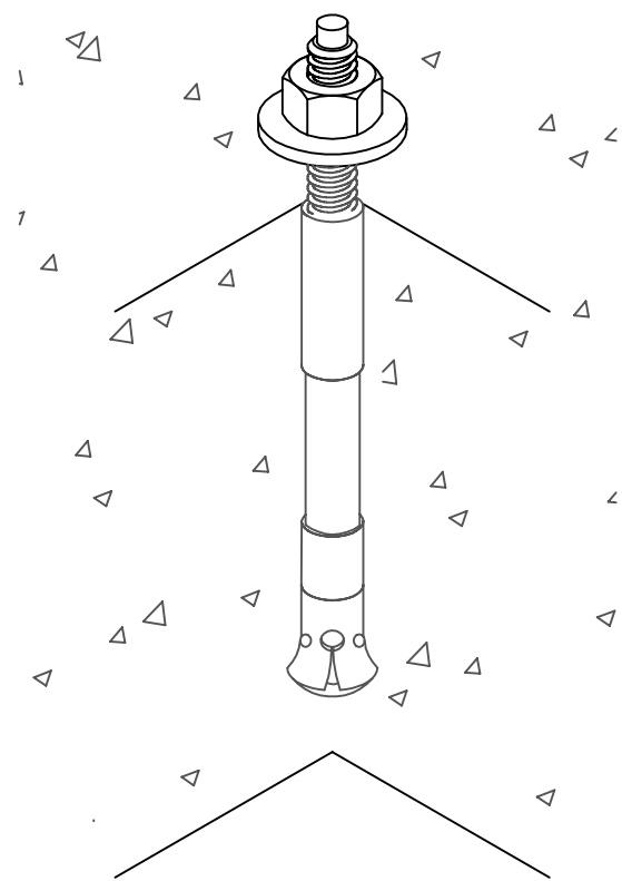
KUAB ANCHOR BOLT SEISMICALLY RATED UNDERCUT ANCHOR BOLT
