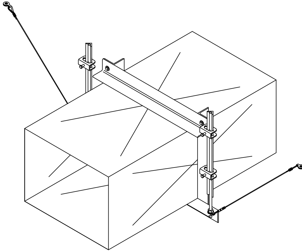
KINETICS MODEL QUAKEKIT-D SEISMIC CABLE RESTRAINT KIT WITH KHRC ROD STIFFENER CLAMPS ASHRAE TYPE J
