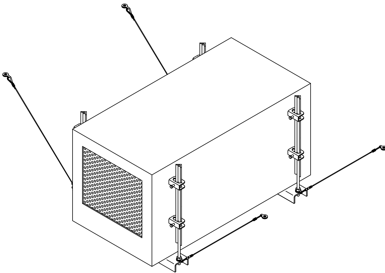
KINETICS MODEL QUAKEKIT-D SEISMIC CABLE RESTRAINT KIT WITH KHRC ROD STIFFENER CLAMPS ASHRAE TYPE J
