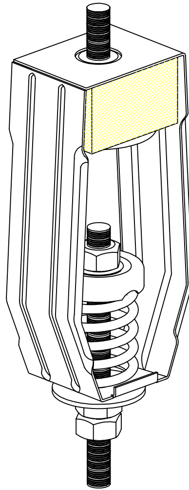
SFH SPRING HANGER ASHRAE TYPE 3
