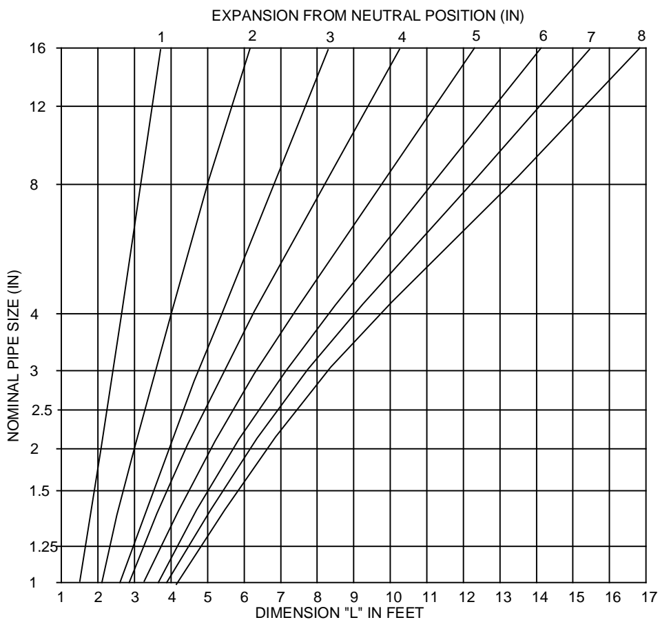
EXPANSION LOOP CAPACITY FOR CARBON STEEL PIPES
