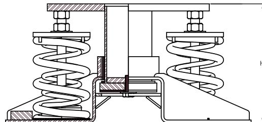
Four (4) Spring Housing Example
