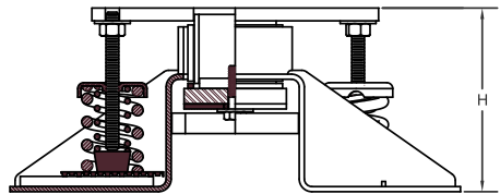
Two (2) Spring Housing Example
