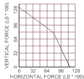
SEISMIC CAPACITY (ASD)
