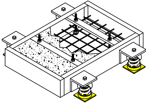
CIB-H CONCRETE INERTIA BASE ASHRAE TYPE C
