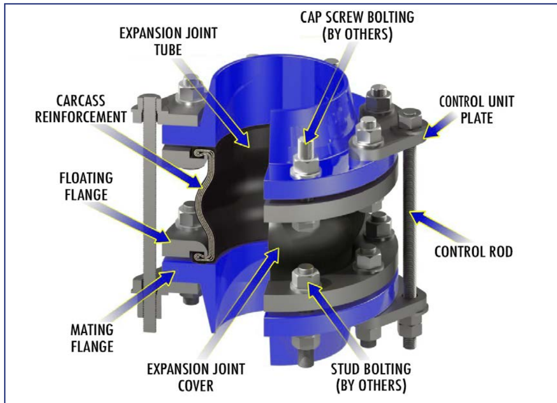
Shown as KINFLEX FC Single Arch Design with Limit Rod (Figure 1)
