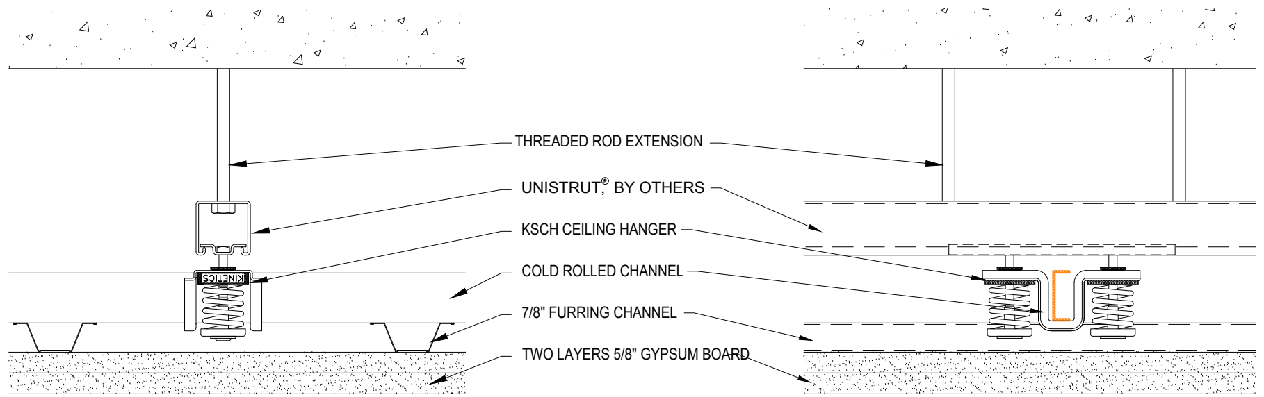
TRAPEZE UNISTRUT® AS REQUIRED
