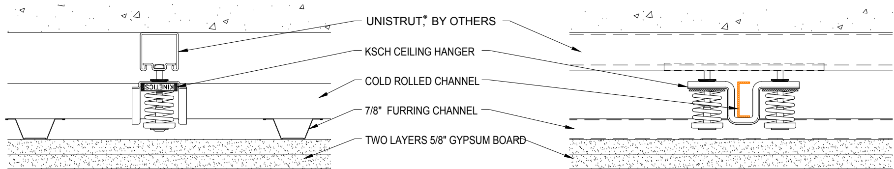
UNISTRUT® ATTACHED TO DECK
