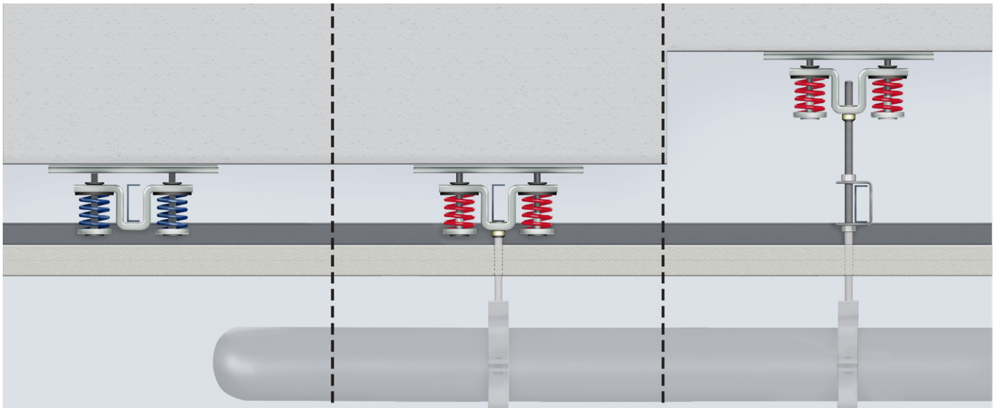
Standard Configuration: Simple ceiling with fixed airspace
