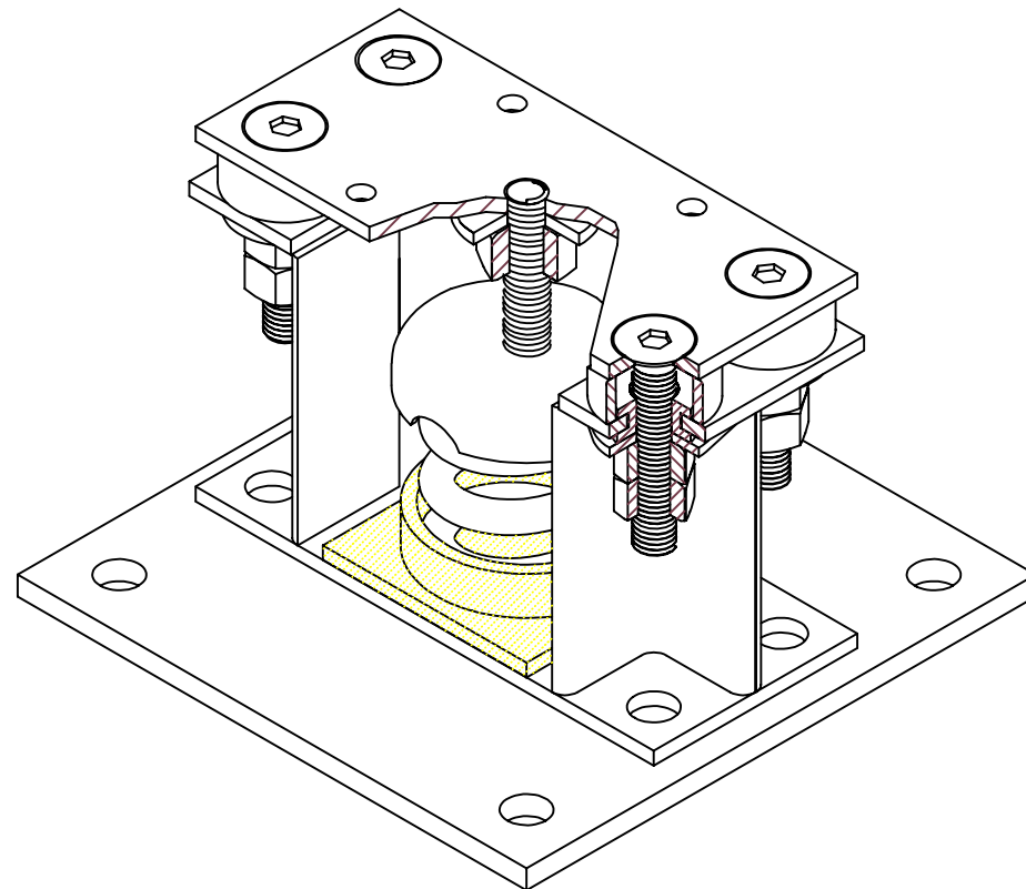
FLSS ISOLATOR WITH OPTIONAL OVERSIZED BASEPLATE ASHRAE TYPE 4
