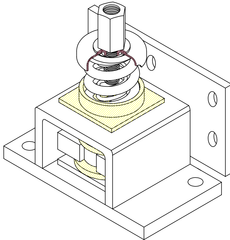
FMS ISOLATOR ASHRAE TYPE 4
