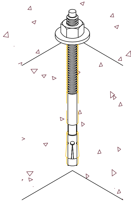
KCAB ANCHOR BOLT SEISMICALLY RATED WEDGE ANCHOR BOLT
