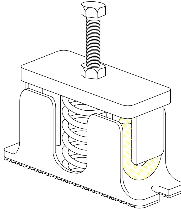
SL ISOLATOR ASHRAE TYPE 3
