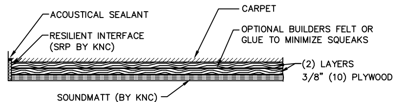
CARPET
