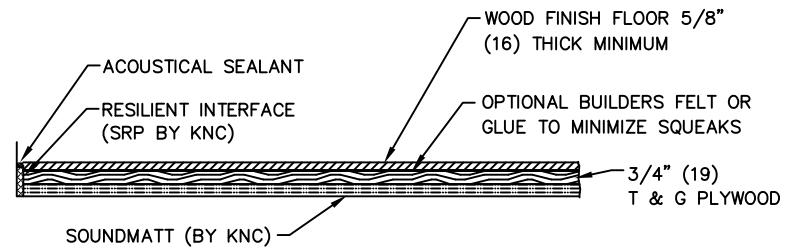
HARDWOOD FLOOR
