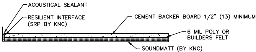
REINFORCED CEMENT BACKERBOARD
