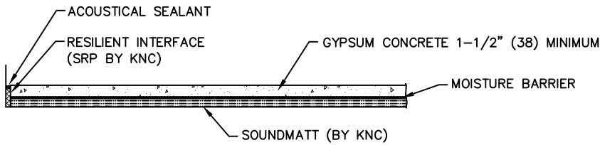
GYPSUM CONCRETE
