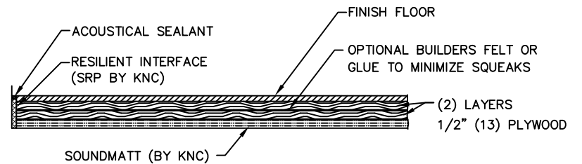
LAMINATE/ENGINEERED WOOD FLOOR
