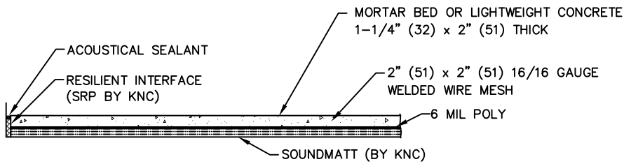
WIRE REINFORCED MORTAR BED, LIGHTWEIGHT CONCRETE
