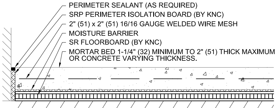
WIRE REINFORCED MORTAR BED OR CONCRETE
