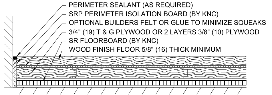
NAIL OR GLUE DOWN HARDWOOD FLOOR
