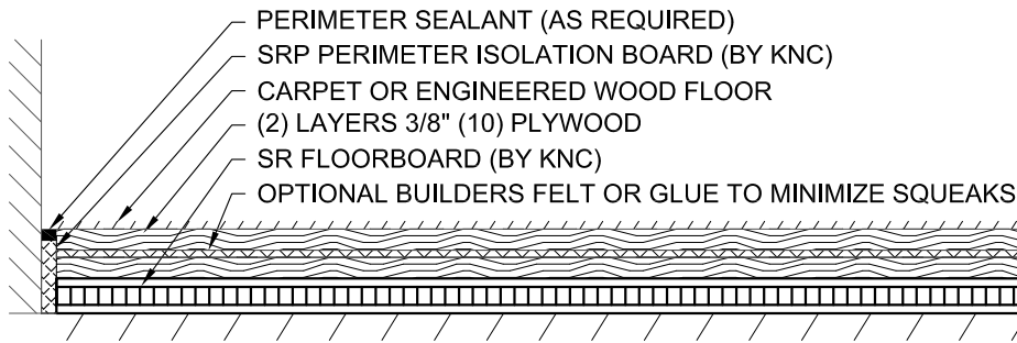
CARPET OR ENGINEERED WOOD FLOOR
