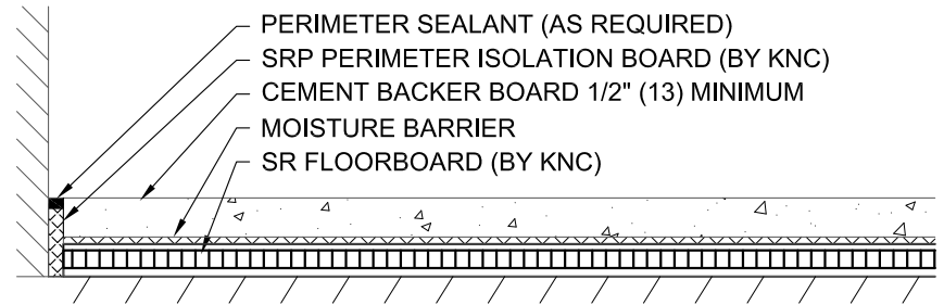
REINFORCED CEMENT BACKERBOARD
