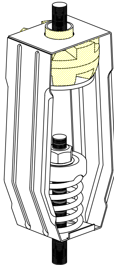
SRH SPRING HANGER ASHRAE TYPE 3
