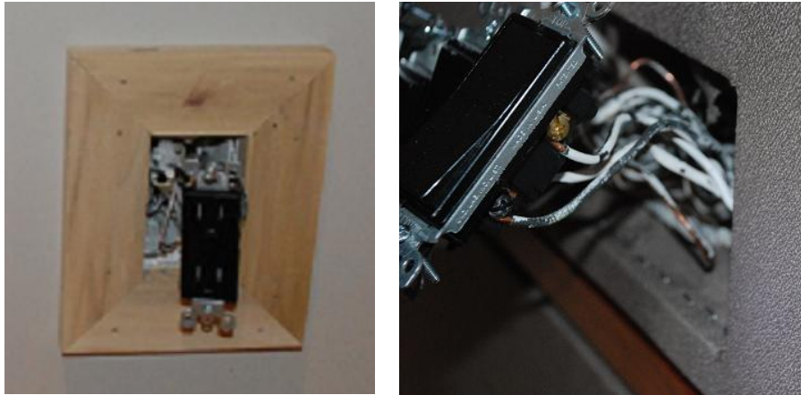
Typical electrical outlet blocking and fabric finish
