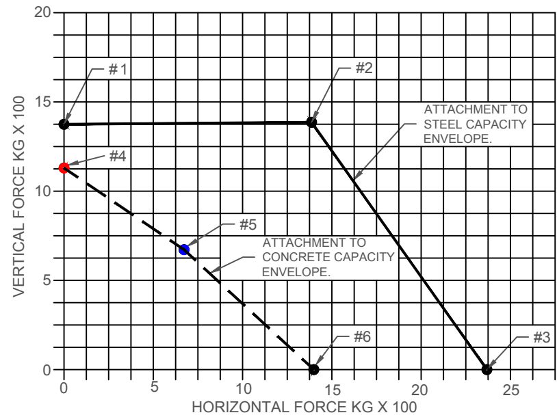
FIGURE 1 RESTRAINT CAPACITY ENVELOPE
