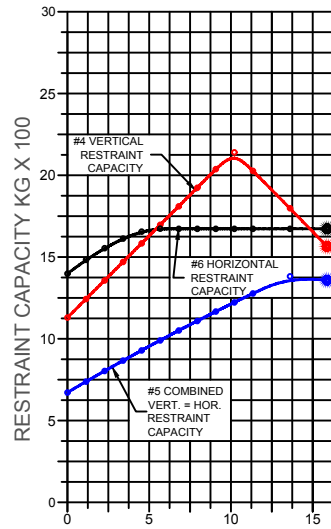
FIGURE 3 CONCRETE ATTACHMENT
