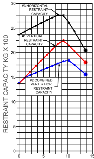
FIGURE 2 STEEL ATTACHMENT
