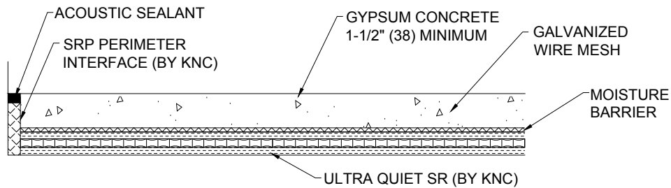
GYPSUM CONCRETE - OPTION B
