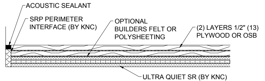
PLYWOOD OR OSB - OPTION C
